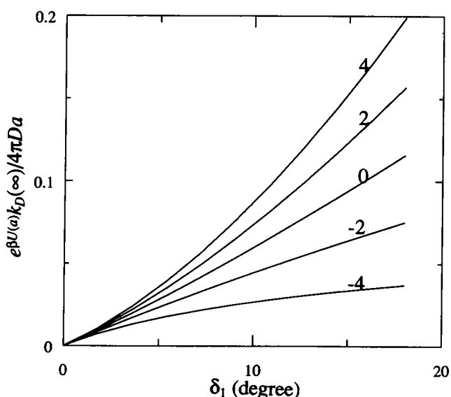
FIGURE 4 The rate constant, scaled by the contact potential, of a uniformly reactive sphere diffusing toward an immobile patched sphere in the Coulombic potential as a function of the patch size. The magnitude of the contact potential, \beta U(a) , is shown above the curves.
