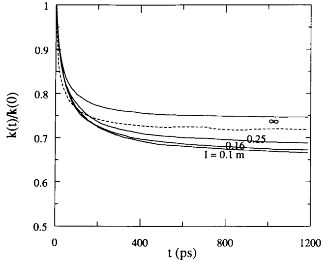
FIGURE 7 The time-dependent rate coefficient, scaled by its initial value, at four ionic strengths. The dashed curve shows the rate coefficient in the radiation boundary limit when the ionic strength is infinite.
