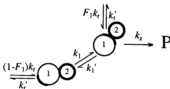
FIGURE 2 The quasichemical scheme when one protein is uniformly reactive.
